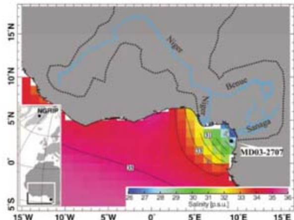
Fig. 1. Annual SSS in the Gulf of Guinea (8). Location of MD03-2707 (02°30.11'N, 09°23.68'E, 1295 m water depth) and drainage basin of Niger and Sanaga rivers (delineated by dotted line) are indicated. The Sanaga River, with an annual discharge of 77 km 3 , drains a basin of 158,000 km 2 with the highest precipitation (10 mm/day) in the African continent (23); the catchment of the Niger River (2,400,000 km 2 ) integrates the largest part of WA monsoon area with annual runoff of almost 200 km 3 [data from Global Runoff Data Centre ( http://grdc.bafg.de )].
